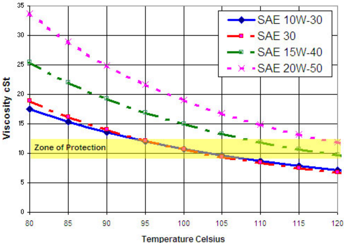
Viscosity Curve
